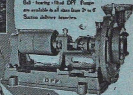
'DPF' BELT DRIVE PUMP
