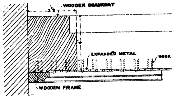
DETAILS AT C. PLAN Fig. 5
