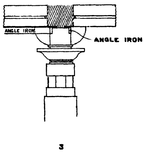
OTHER DEVICES FOR SUPPORTING BROKEN BEAMS (See para. 186).
