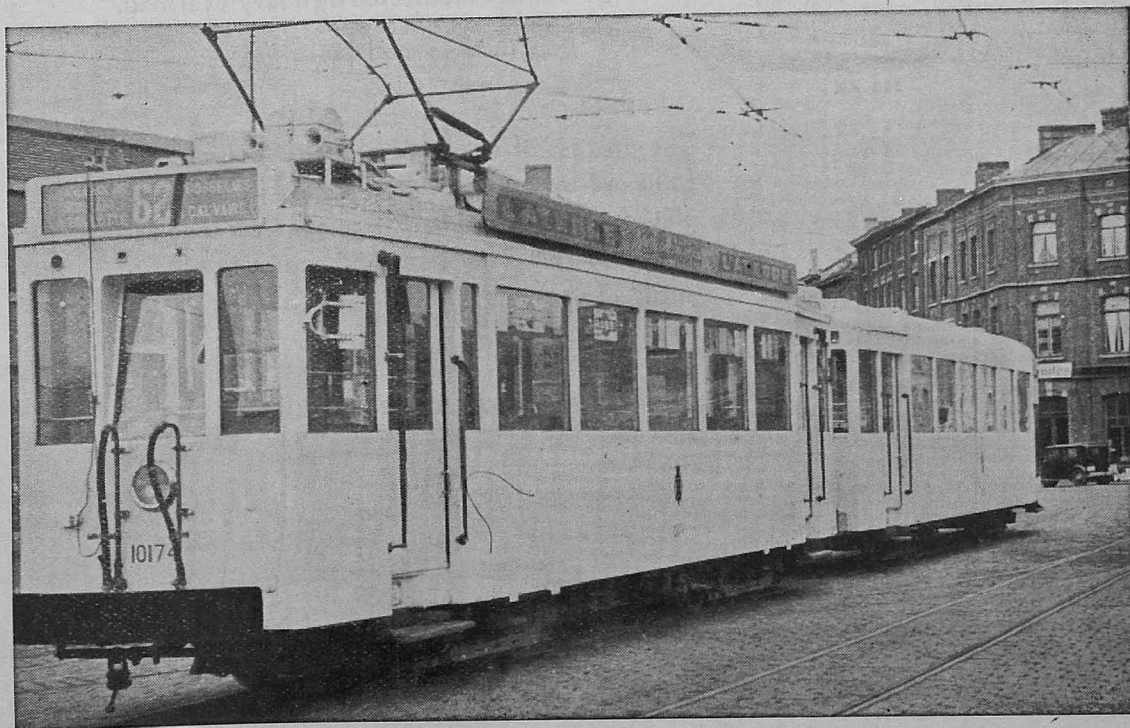
Modern electric train of the Belgian Light Railways consisting of motor and trailer car, both of all-metal construction
