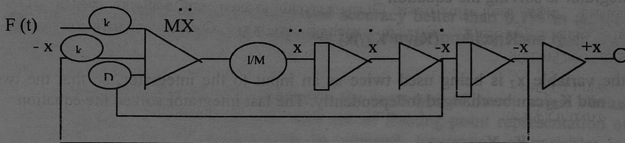
Figure 4-1. Diagram for the automobile suspension problem.
