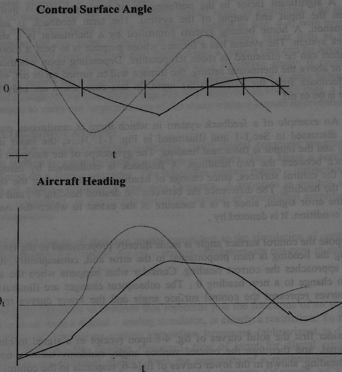
Figure 4-6. Aircraft response to autopilot system.
