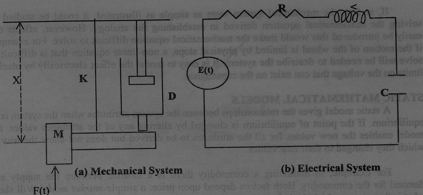
Figure 1.6 Analogy between mechanical and electrical systems
