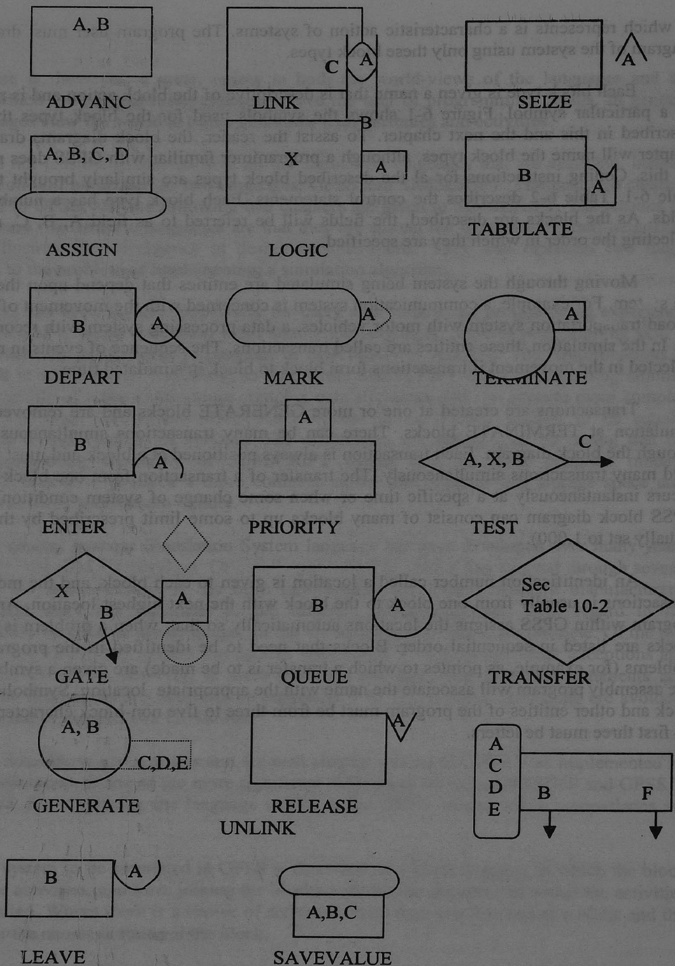
Figure 6-1. GPSS block-diagram symbols.
