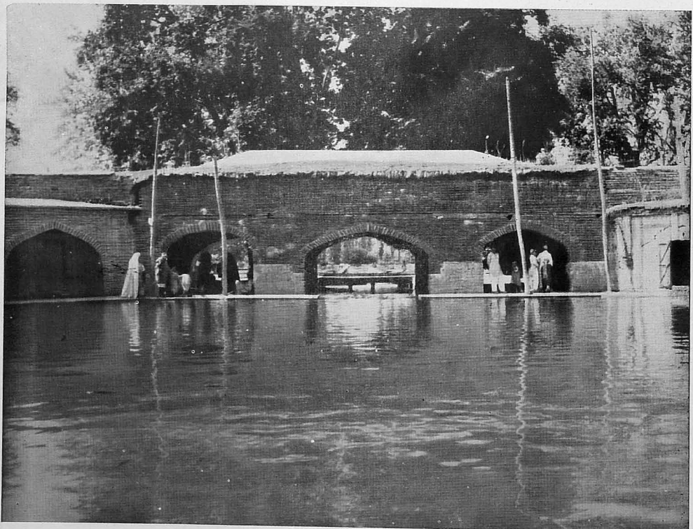
Verinag : Mughal arcade, A, before, and B, during conservation
