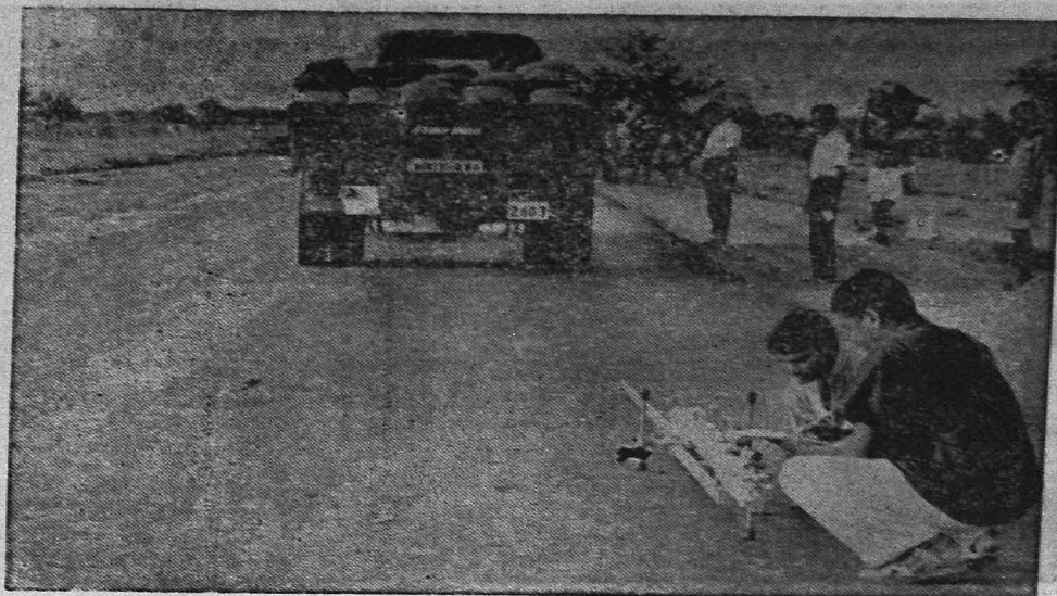
Fig. 2.5.5. Benkelman Beam Deflection Test under a rear axle load of 18000 lbs.
