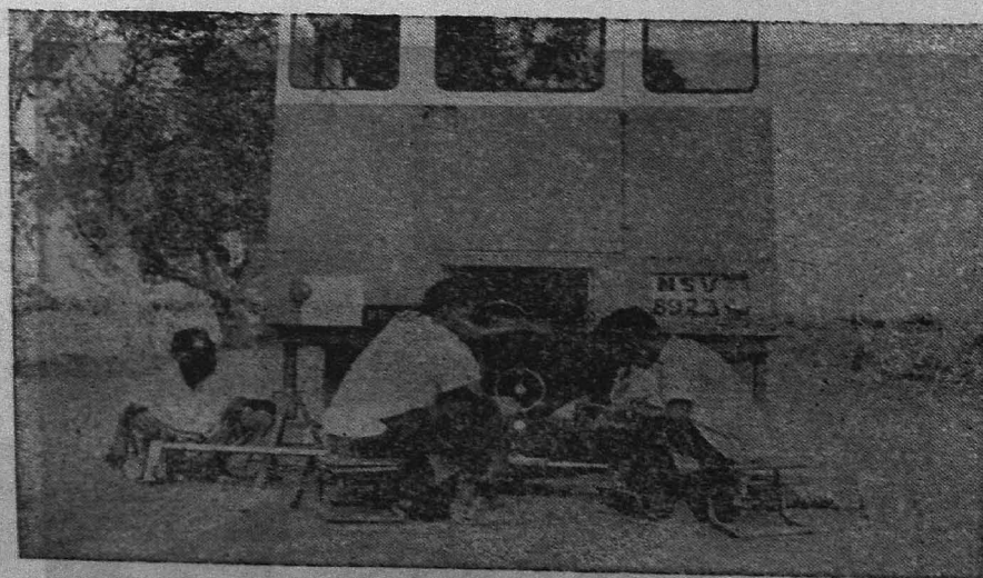
Fig. 2.5.4. In-situ California Bearing Ratio Test in Progress in the distressed site, with the field Laboratory Van of the Highways Research Station, Madras.
